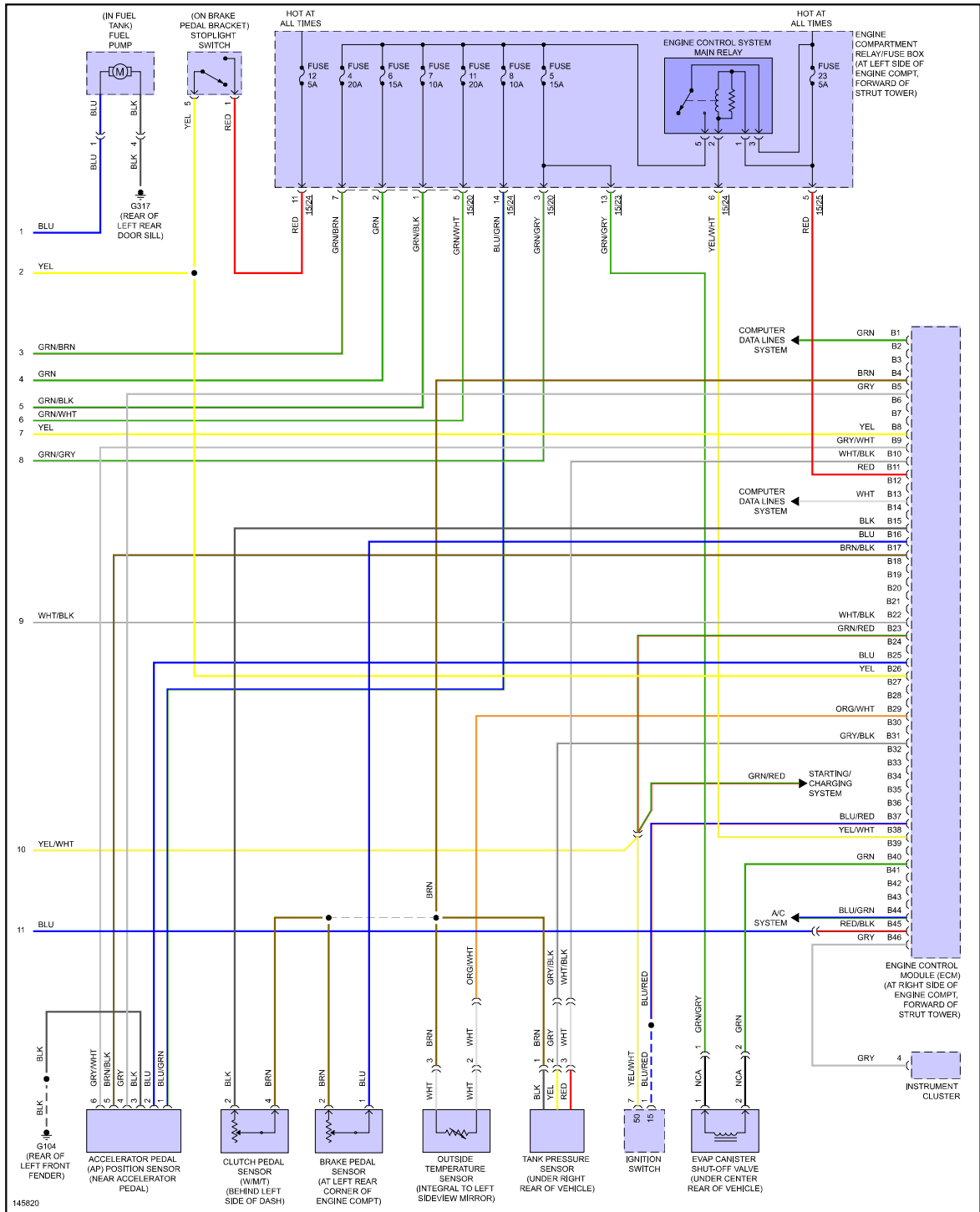
Fig 3: 2.3L Turbo, Engine Performance Circuits (3 of 3)
