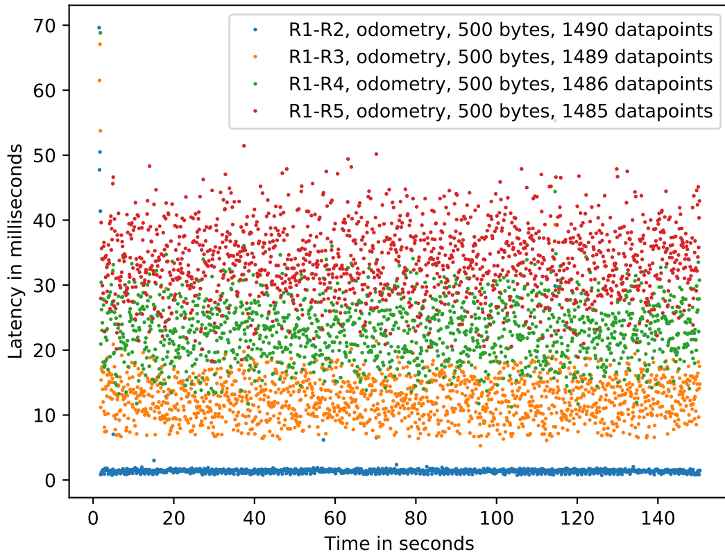
Latency graph for Zhaolin's setup (40 outliers dropped)
