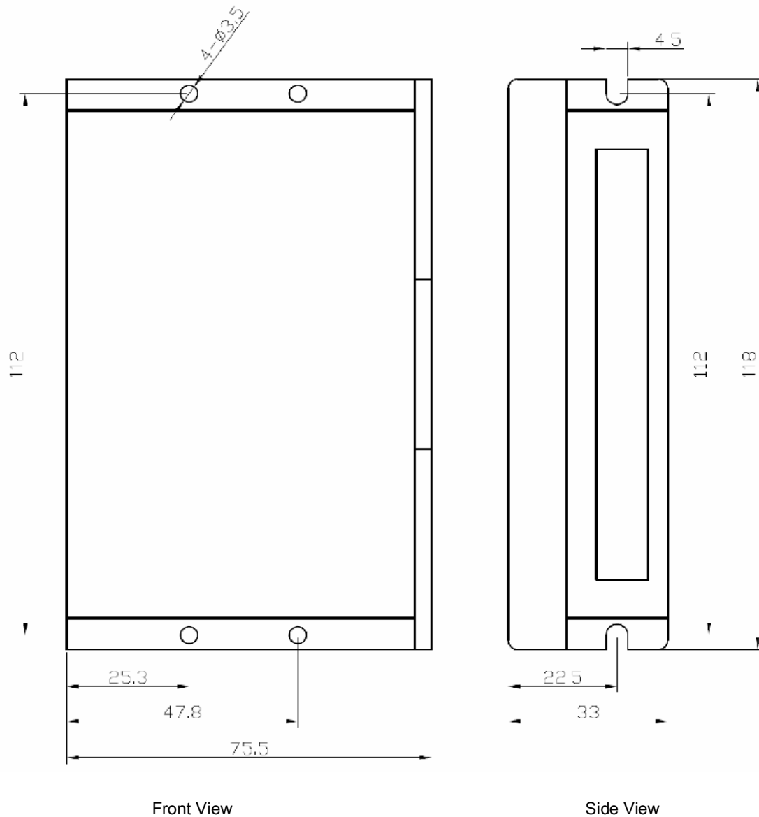
Figure 1: Mechanical specifications
