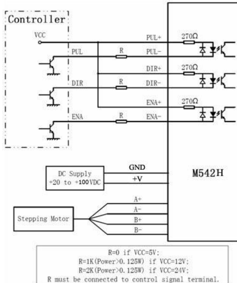
Figure 10: Typical connection
